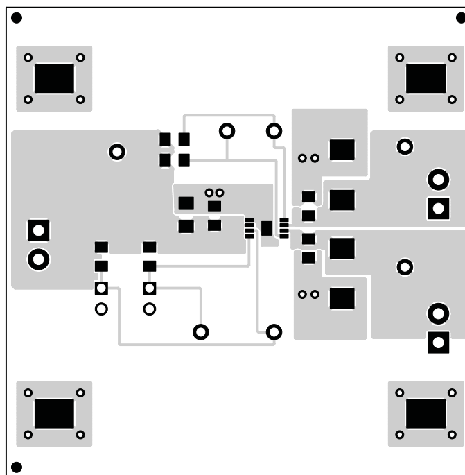
Figure 7. TPS20xxEVM-296 Top-Side Layout
